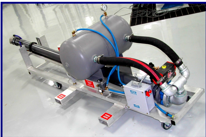
Missile Impact Cannon Photo optic speed measurement, laser targeting, many safety features
